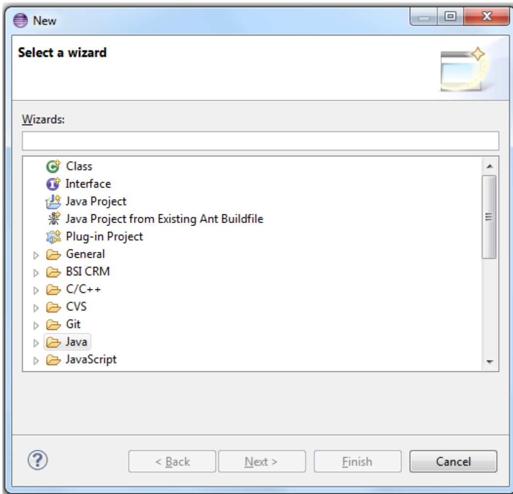
Figure 13. "New" Wizard
