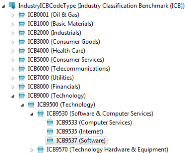
Figure 31. A hierarchical code type class shown in the Scout SDK.
