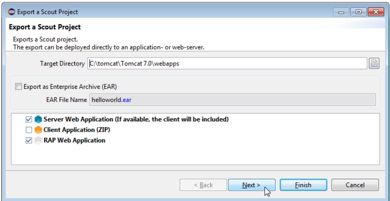
Figure 13. The first dialog of the Export Scout Project wizard. Here, the target directory for the WAR files that will be generated by the wizard is specified.
