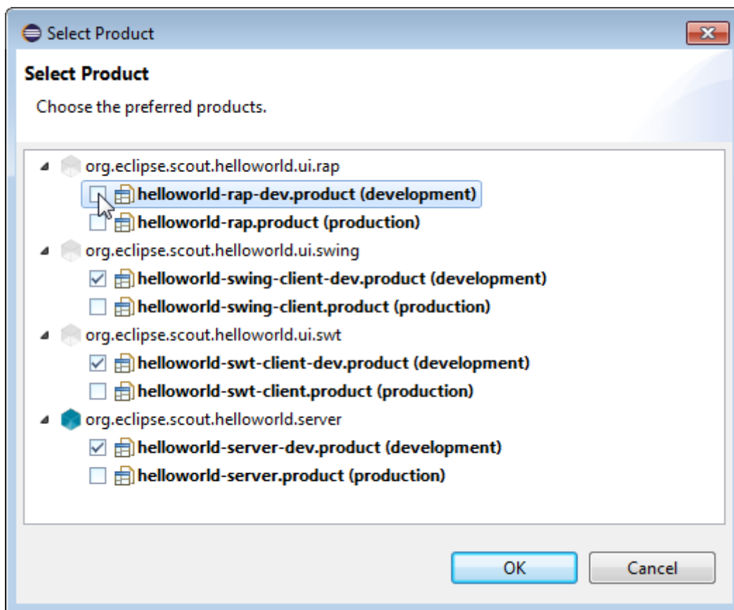
Figure 22. Using the Edit Content... icon shown on the left hand side, the product selection dialog shown on the right side is opened. Using this product selection dialog, the list of launcher boxes can be
