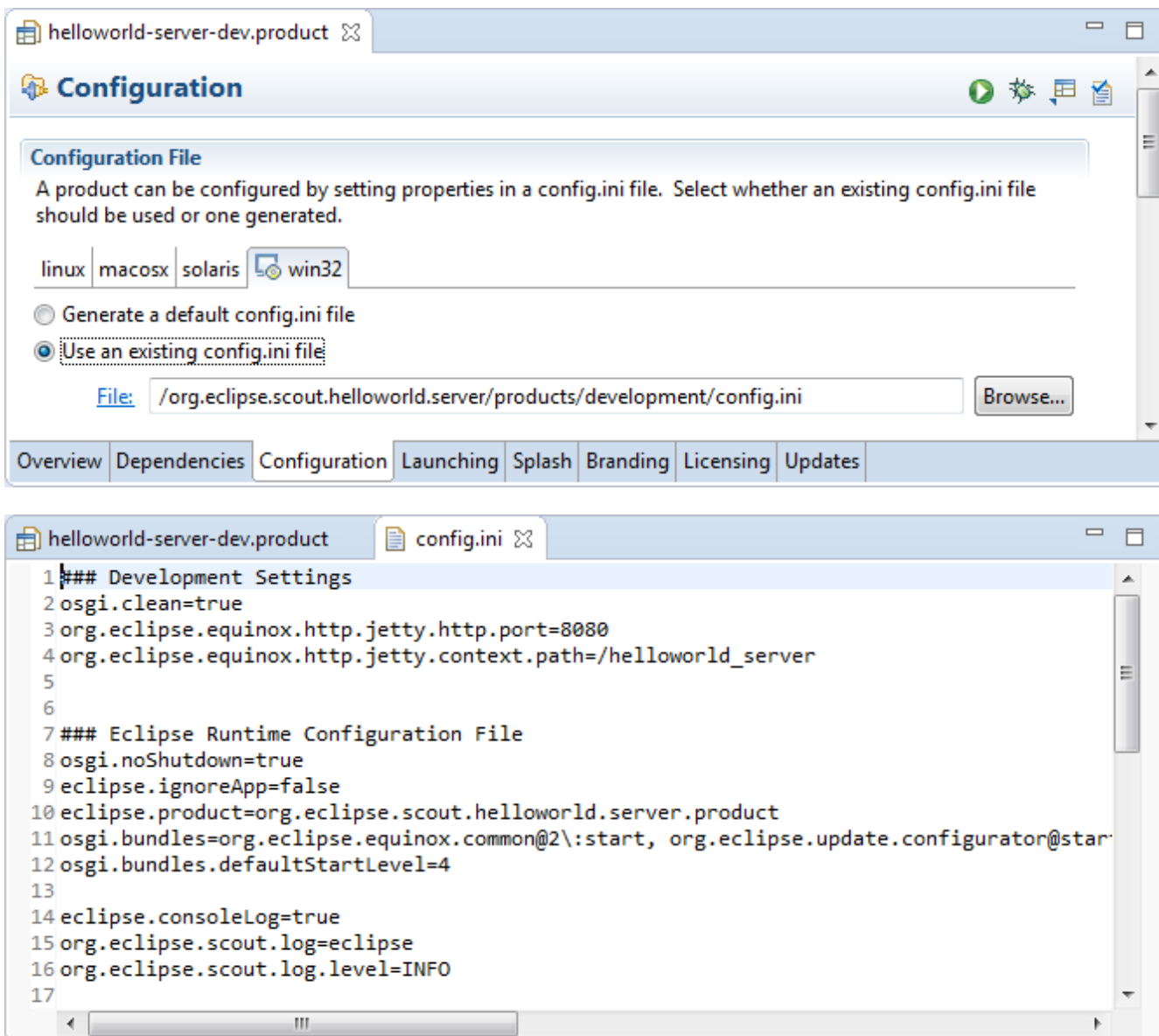
Figure 25. Above, the definition of the products config.ini in tab Configuration of the product file editor. Below, the content of the configuration file of the “Hello World” server application is provided in a normal text editor.
