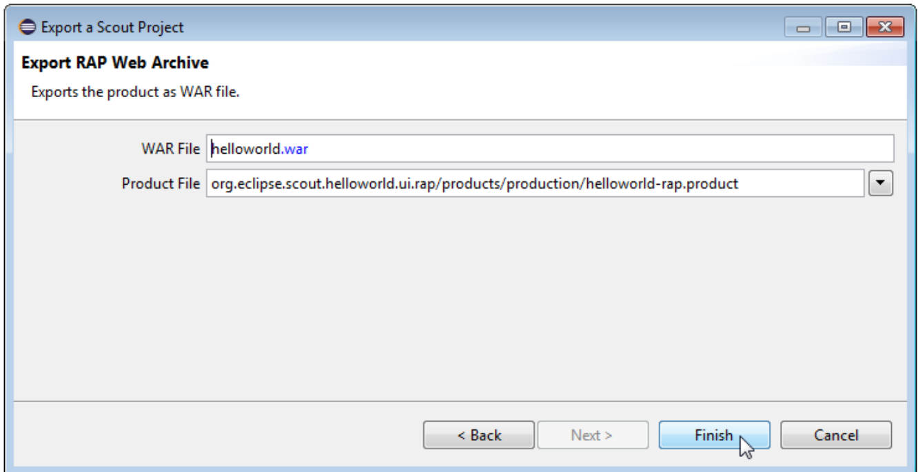
Figure 15. The last dialog of the Export Scout Project wizard defines the export of the RAP server. Normally, the proposed field values do not need any adjustments.
