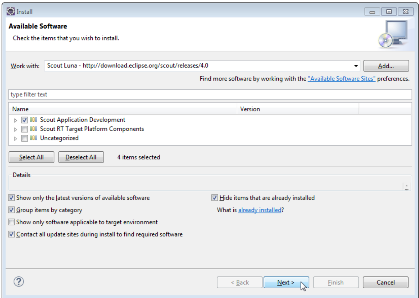
Figure 61. Select the Scout features to add to the Eclipse installation
