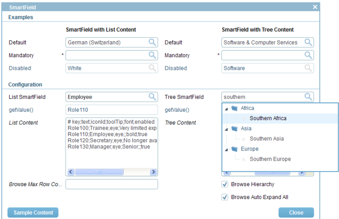
Figure 42. Smart field examples. Smart fields support “search-as-you-type” and are used to select a value from of a list of elements or a tree.
