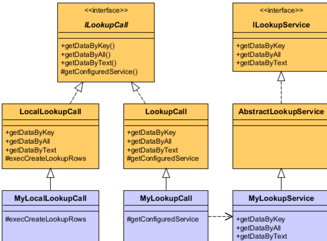
Figure 32. Implementing a lookup call with a corresponding lookup service. Scout framework components are shown in orange, user code in blue.
