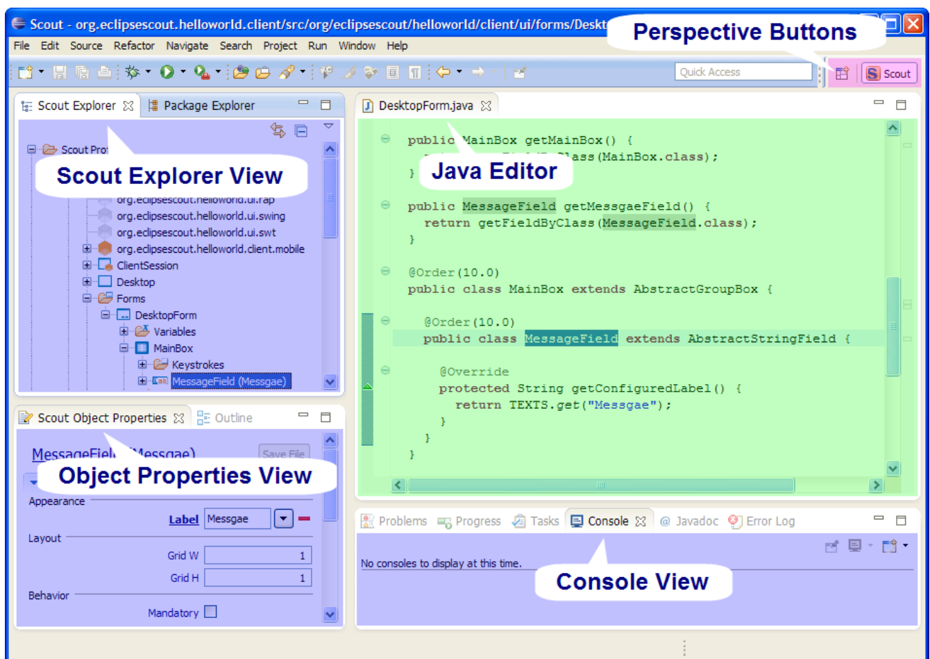
Figure 64. The Eclipse IDE with the Scout perspective. The colors indicate the different elements. View parts (blue), editor parts (green) and perspective buttons (purple).
