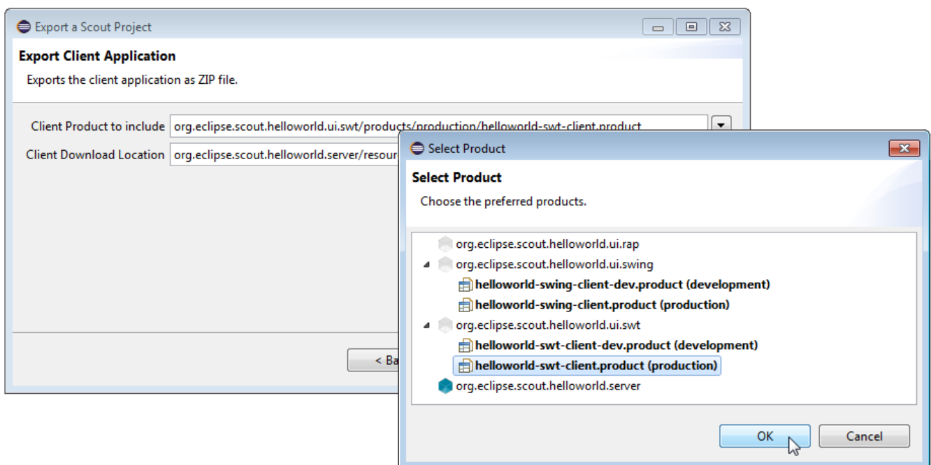
Figure 14. The third dialog of the Export Scout Project wizard defines the client application to be included in the helloworld_server.war file. In the last step of the export wizard the RAP sever is
