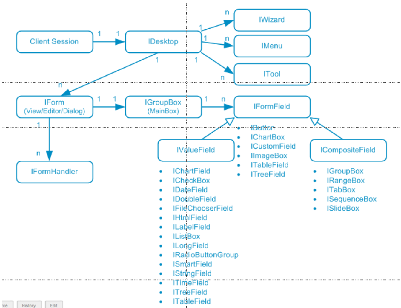
Figure 33. A class diagram for the Scout's client model
