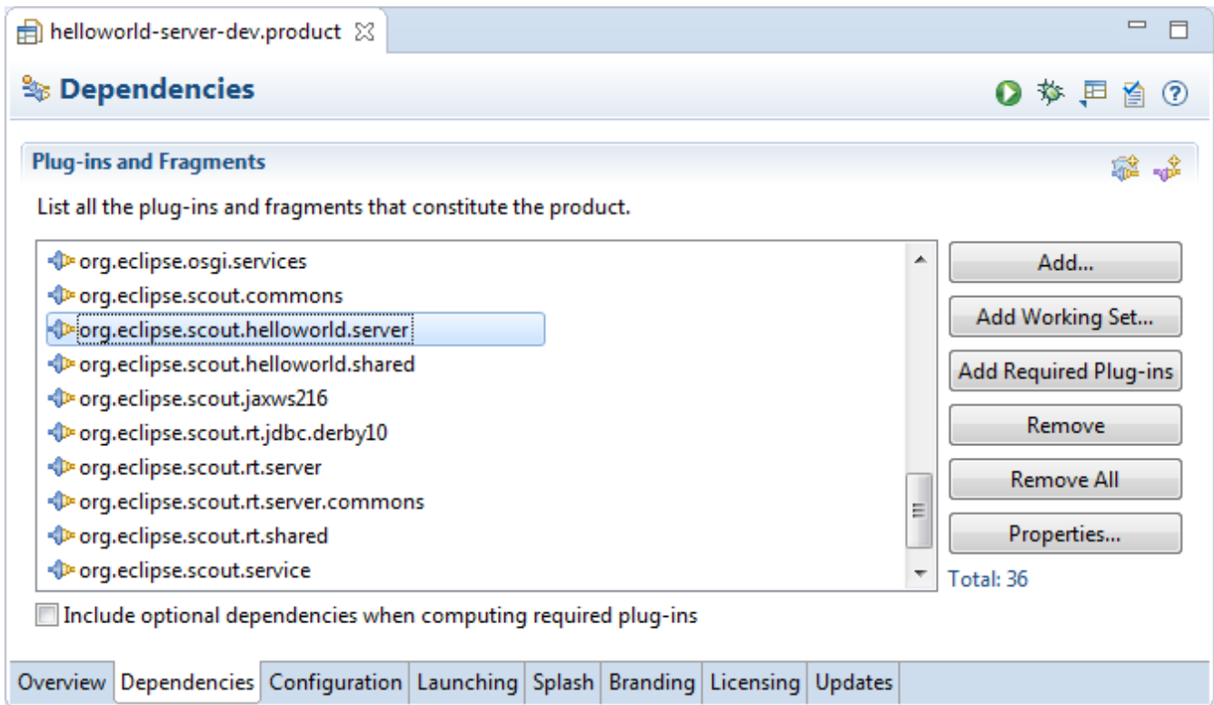
Figure 24. The Eclipse product file editor showing file helloworld-server-dev.product of the “Hello World” application. In the Dependencies tab shown above, the list of Eclipse plugins that are required for the server application are shown.
