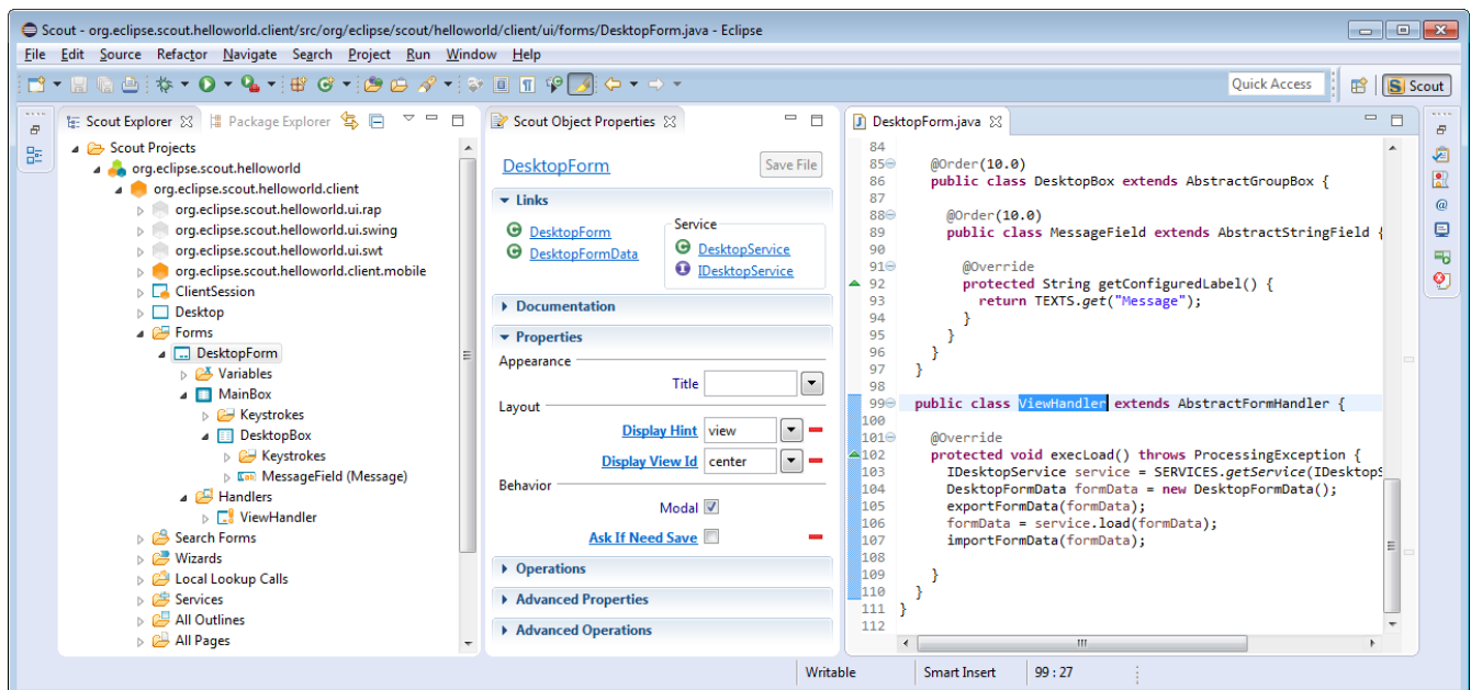
Figure 21. Scout SDK showing the DesktopForm 's ViewHandler in the Scout Explorer and the properties of the DesktopForm in the Scout Object Properties.
