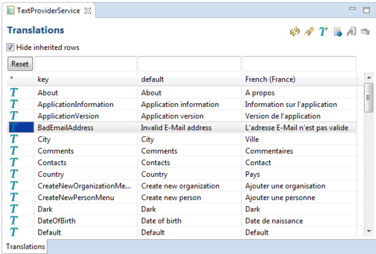
Figure 26. The NLS editor provided by the Scout SDK. This editor is opened via the Open NLS Editor ... link in the Scout Object Properties of the HelloWorldTextProviderService node.
