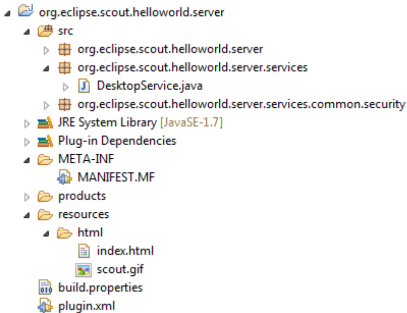
Figure 30. The “Hello World” server plugin shown in the Eclipse package explorer. The files for the download page are located under resources/html.
