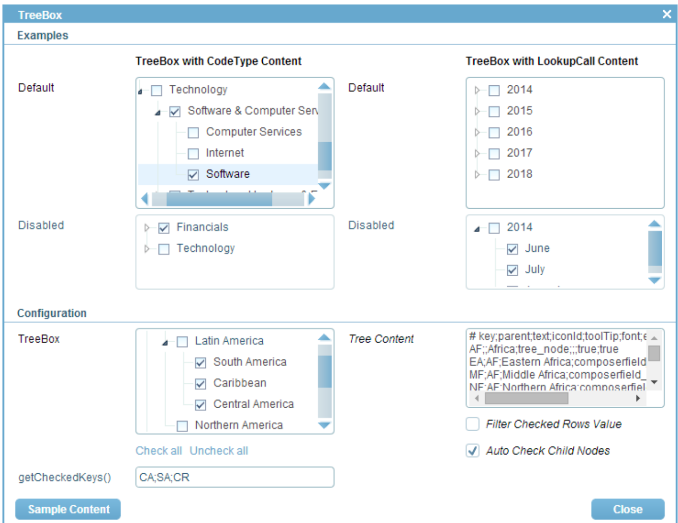
Figure 41. Tree box fields displaying elements defined by hierarchical code types and lookup calls.
