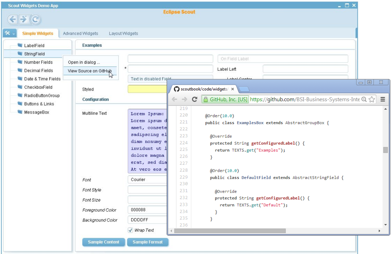
Figure 34. The "Scout Widgets Demo App". The widgets demo application features examples of the most commonly used Scout widgets. For each widget shown, example use cases are presented in a individual form. As shown in the screenshot, the corresponding Scout source code is made available via the View Source on GitHub context menu.
