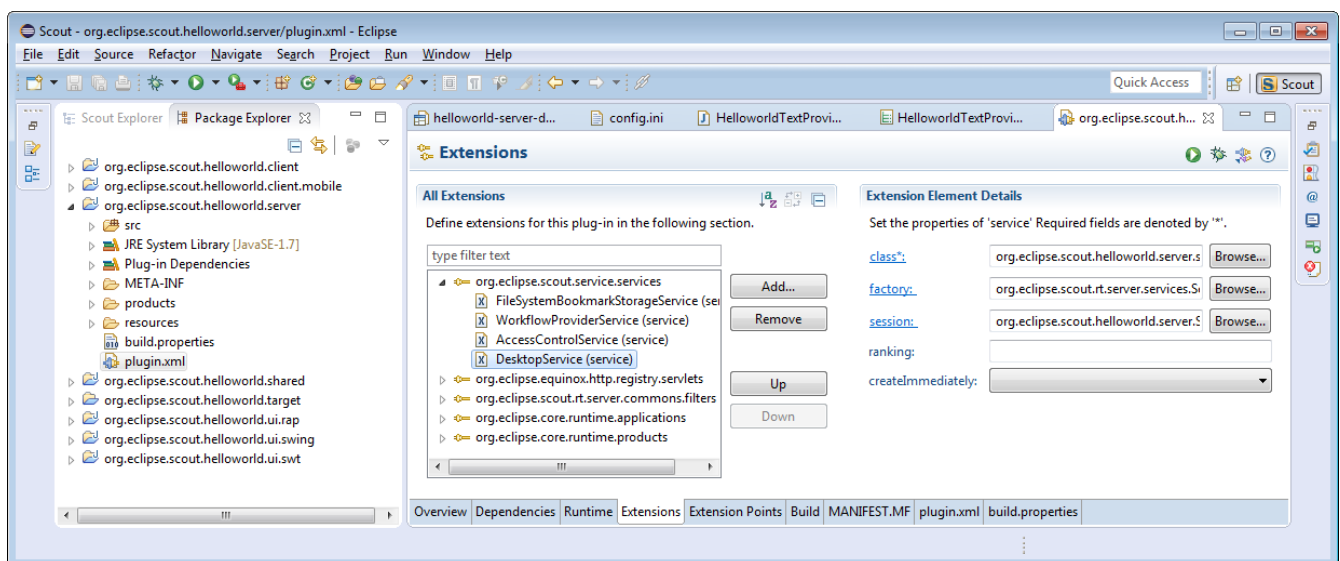
Figure 27. The Eclipse plugin editor for plugin.xml files. In the tab Extensions the "Hello World" desktop service is registered under the extension point org.eclipse.scout.service.services.
