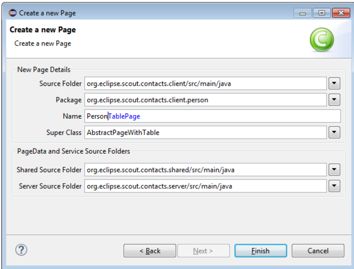
Figure 34. Add the person page to the "Contacts" application.
