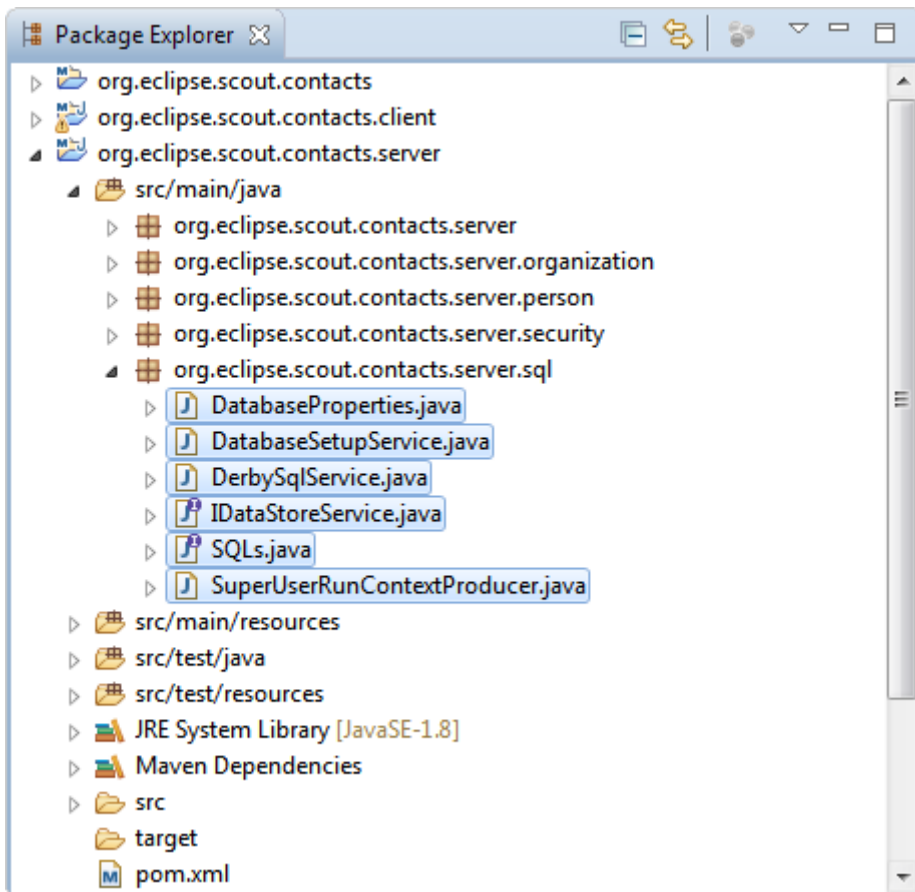
Figure 39. The copied database classes in the tutorial workspace.
