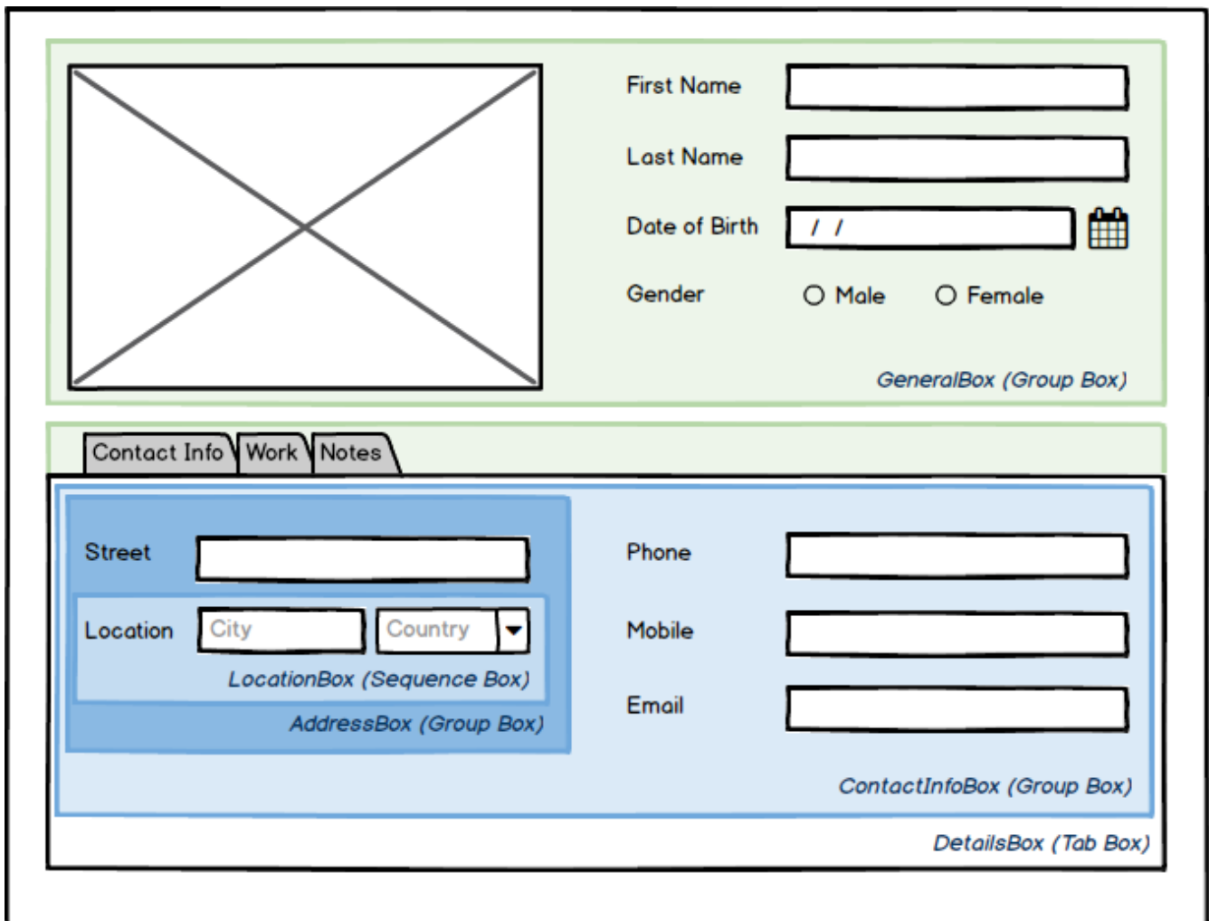
Figure 43. The hierarchical organization of the form including Scout group boxes, tab boxes and a sequence box.
