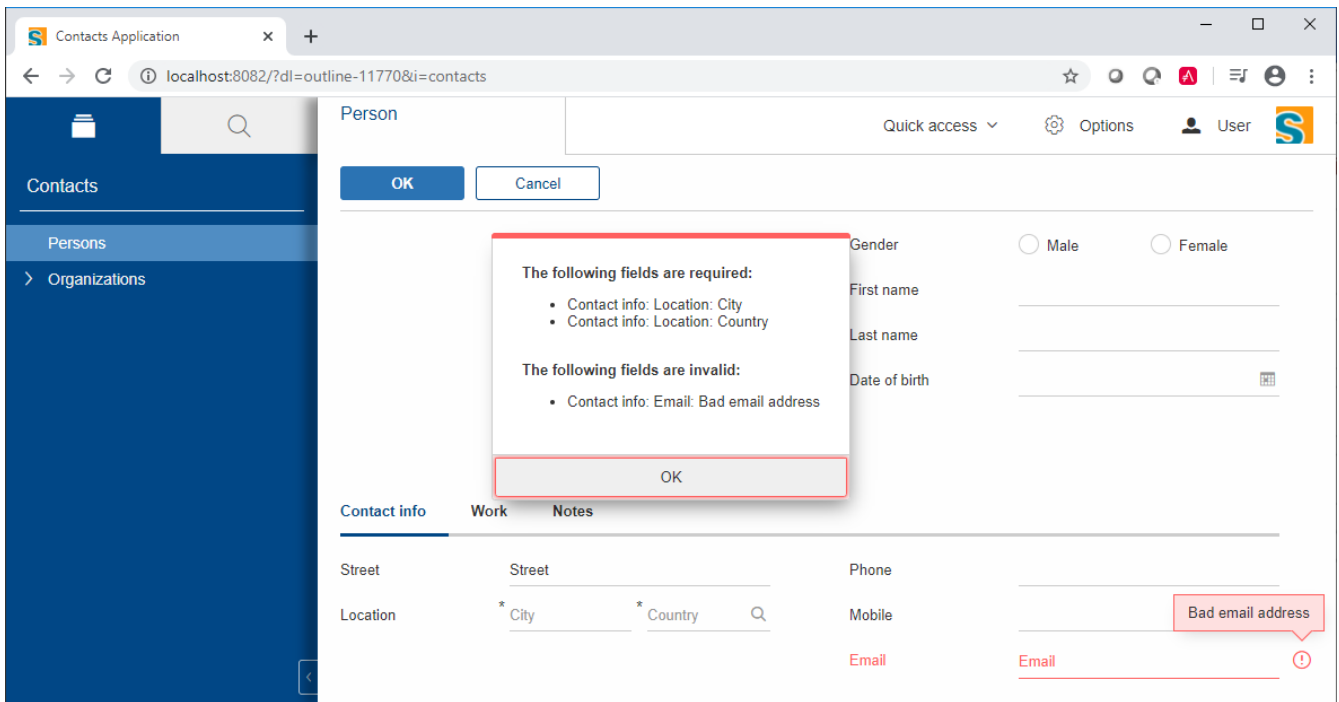
Figure 48. The form field validation implemented for the person form.
