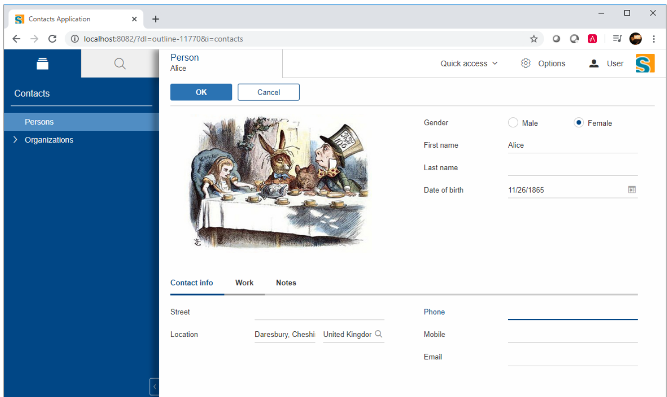
Figure 47. The "Contacts" application with the person form at the end of tutorial step 4.
