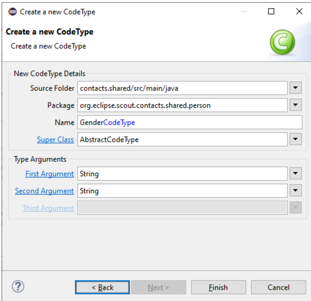
Figure 46. Create the gender code using the Scout new code wizard.
