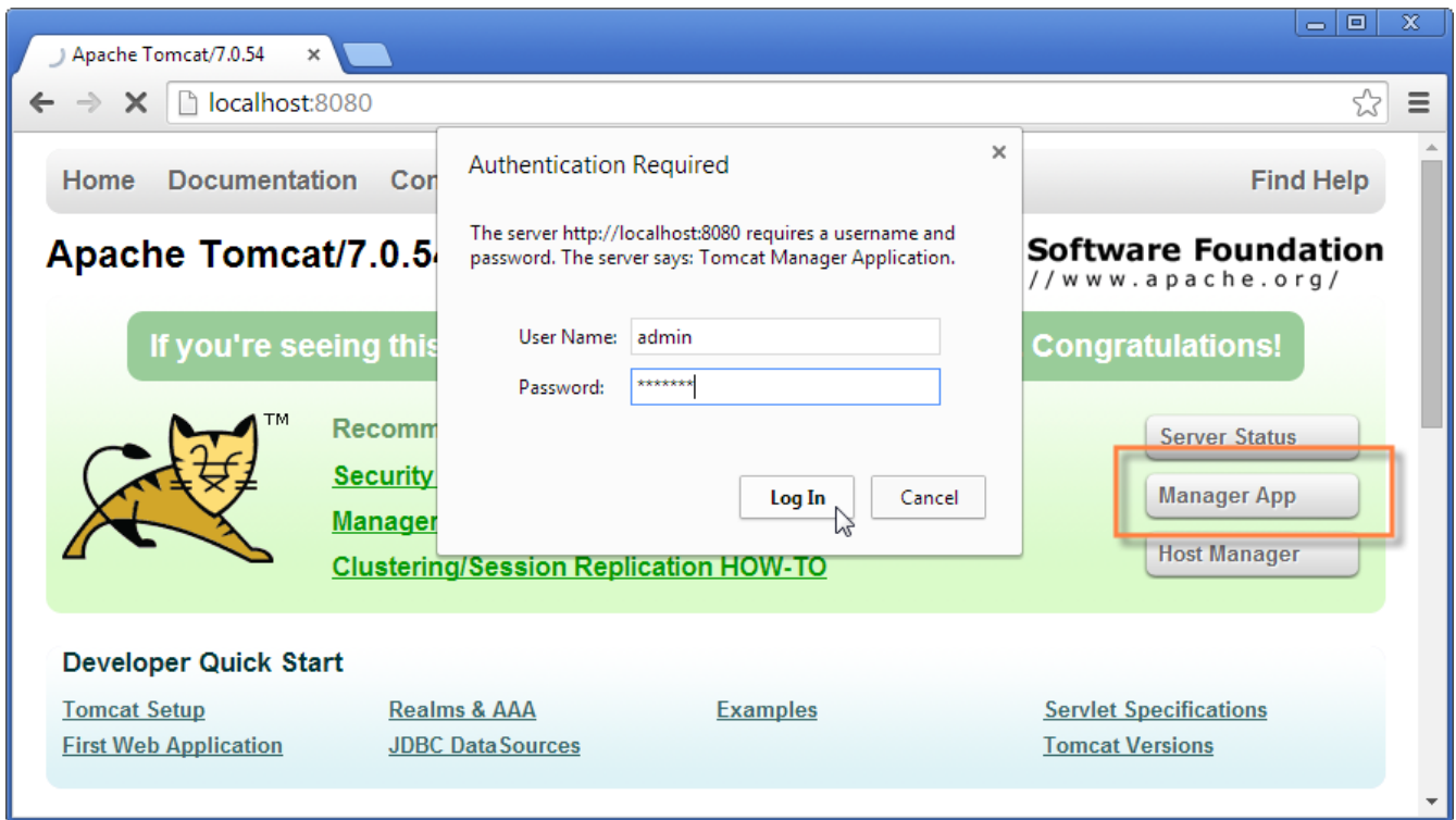
Figure 9. The Tomcat shown after a successful installation. After clicking on the “Manager App” button (highlighted in red) the login box is shown in front. A successful login shows the “Tomcat Web Application Manager”.
