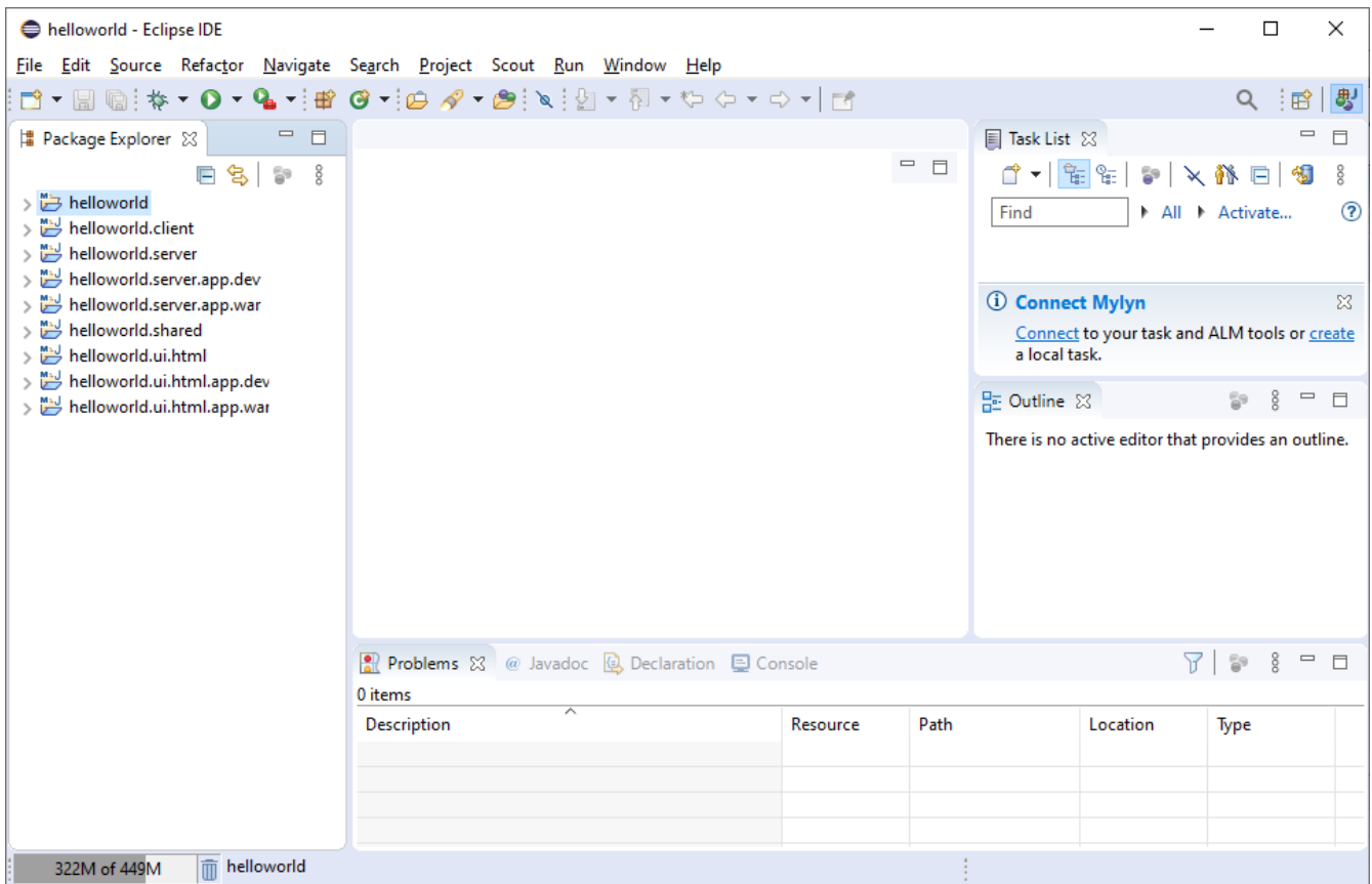
Figure 5. The initial set of Maven modules created for the Hello World application.
