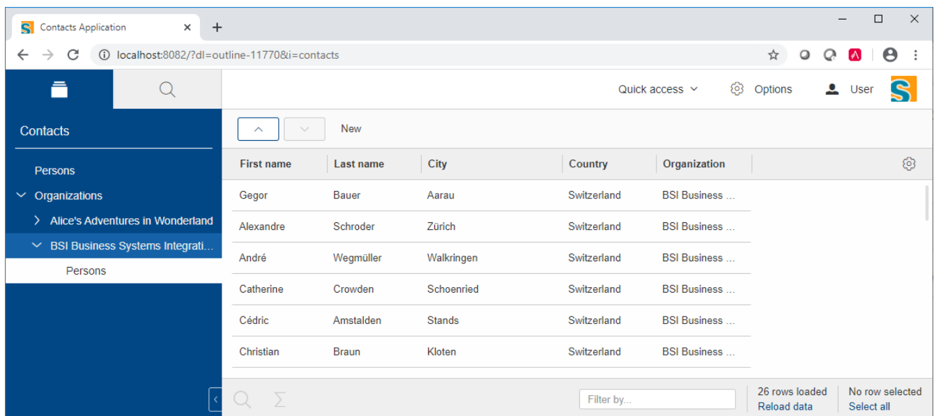
Figure 56. The linked person page only shows persons related to the parent organization page.
