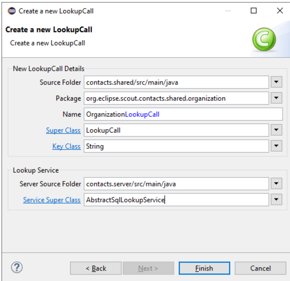
Figure 53. Using the Scout lookup call wizard for creating class OrganizationLookupCall .
