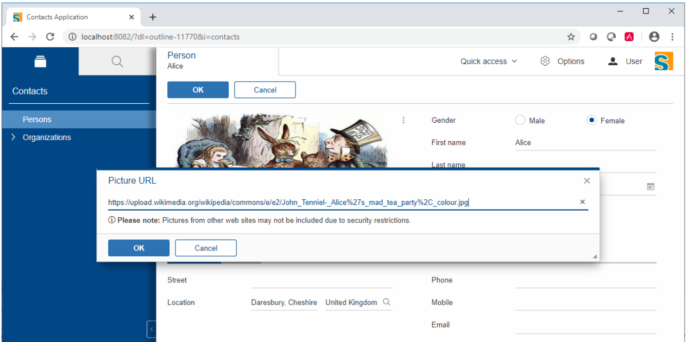
Figure 50. The person form with the refactored picture template field including a menu (red square) and a URL edit form.
