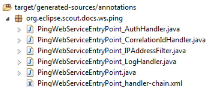
Figure 16. generated artifacts
